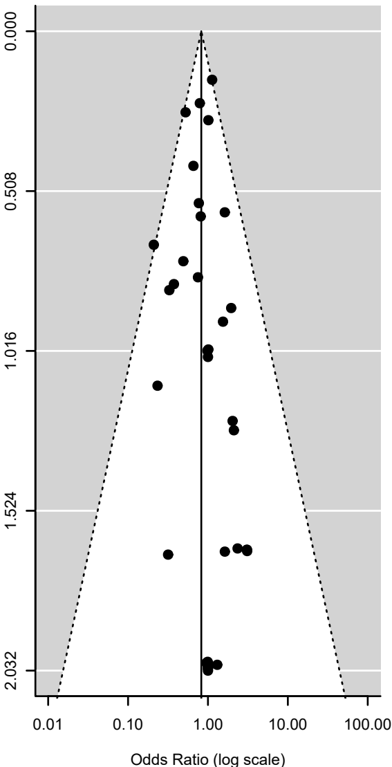
Fig S1: Funnel plot
