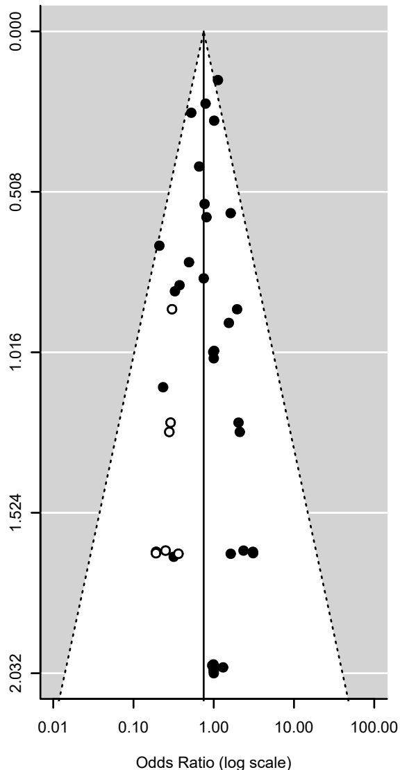
Trim and fill method
