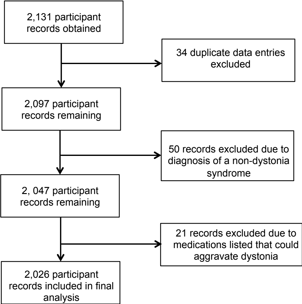
Figure e-1. Data collected from 2,026 individuals for analysis after applying the exclusionary criteria
