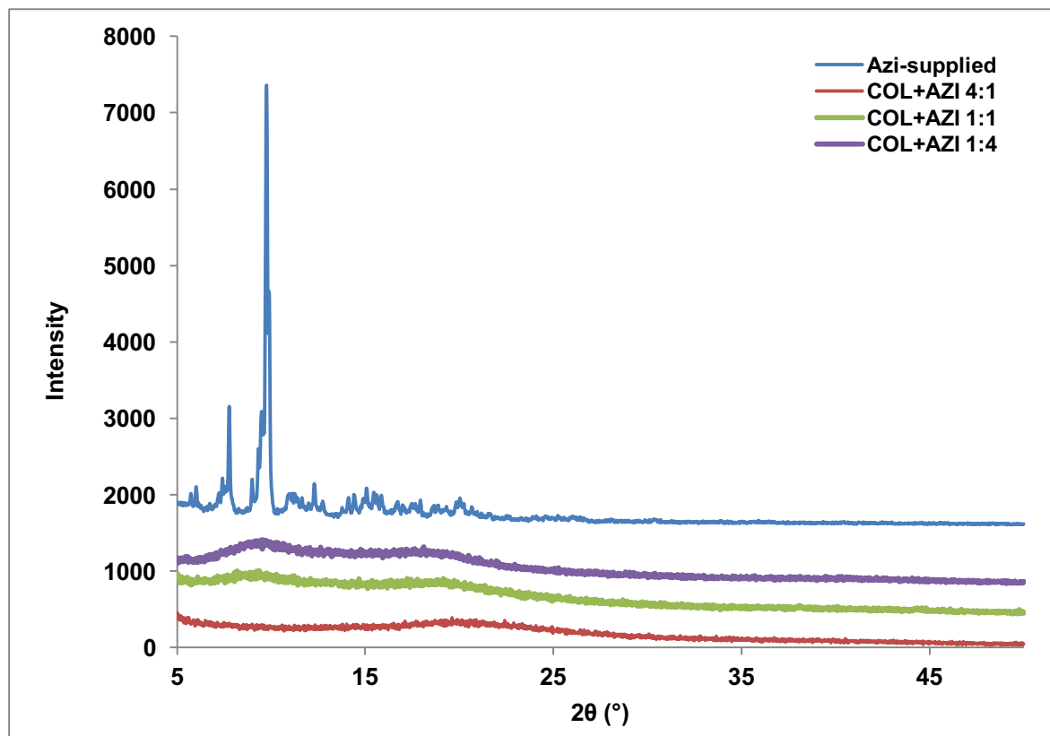
Supplement 1. Powder X-ray diffraction patterns of the spray-dried powder formulations.
