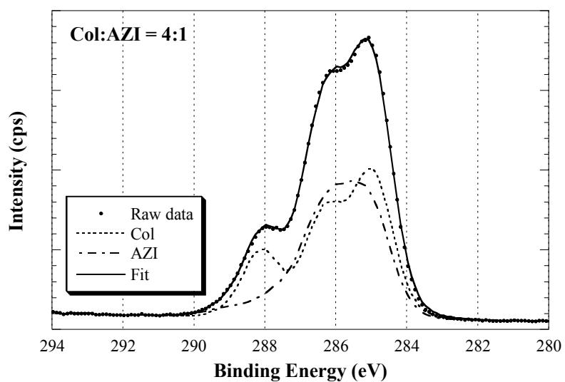
Supplement 2. C 1s high resolution spectrum of composite sample (4Col:1AZI) measured by XPS and two model spectra of the pure compounds (Col, AZI) used for curve-fitting.
