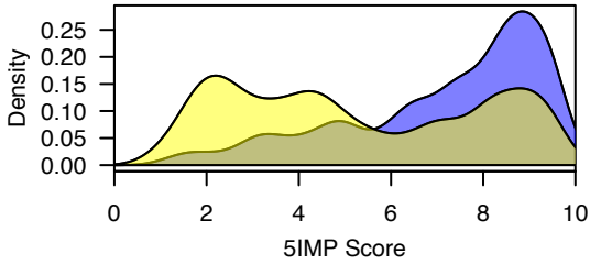
First 99 Coding Nucleotides
