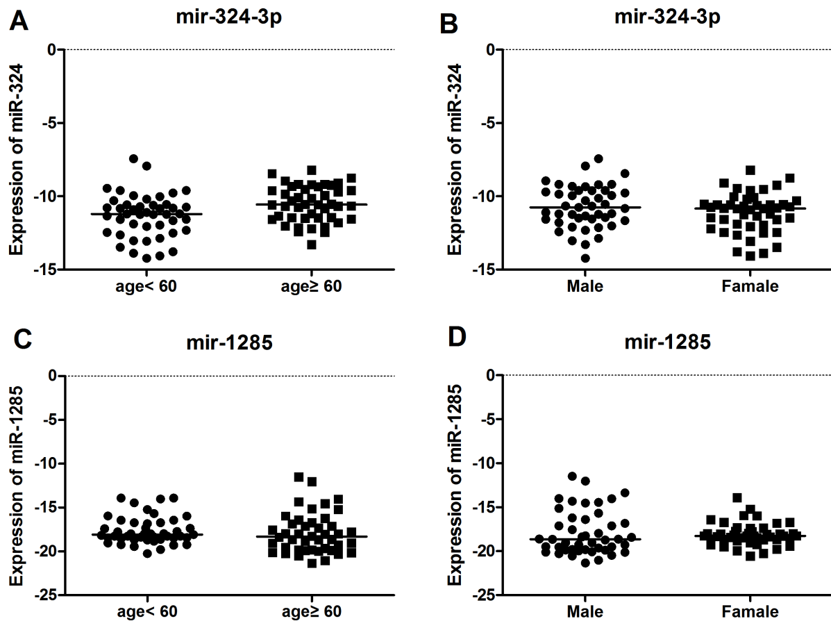
Supplementary Figure S1: The relationship of plasma miRNAs and clinical parameters. LSCC patients were stratified by gender and age. (A) plasma miR-324-3p expression between two age groups; (B) plasma miR-324-3p expression between male and female; (C) plasma miR-1285 expression between two age groups; (D) plasma miR-1285 expression between male and female.
