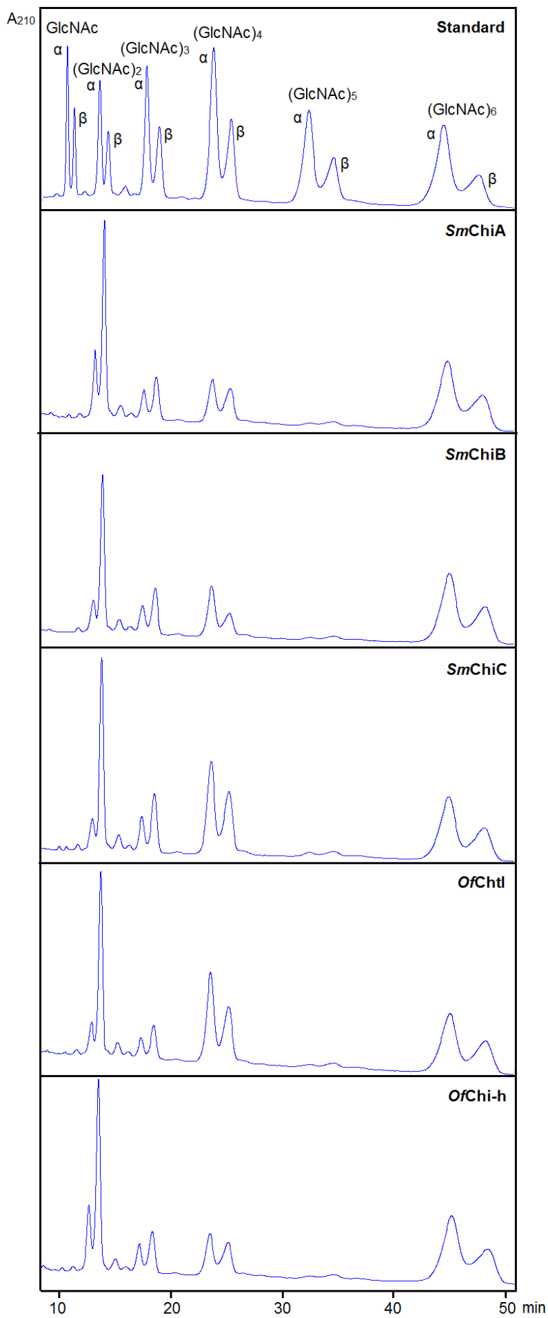
Figure S2. HPLC analysis of the partial products of (GlcNAc) 6 hydrolysis by different chitinases.
