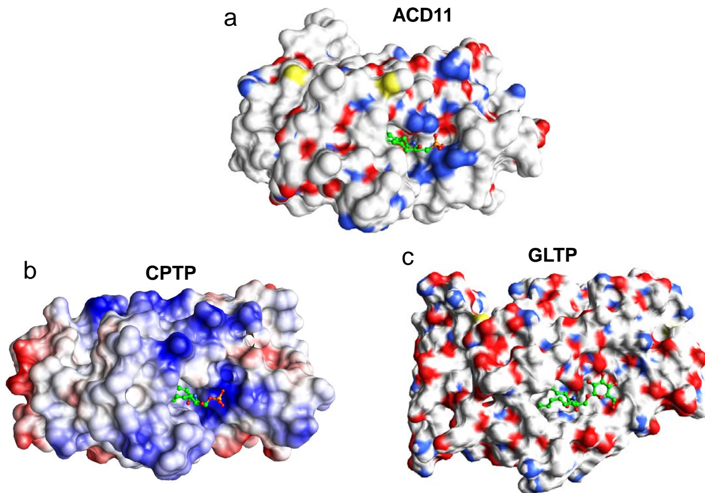
Supplementary Figure S1: Surface electrostatics surrounding the sphingolipid binding site in a) ACD11, b) CPTP, and c) GLTP, respectively. (Blue = cationic; red = anionic; and white = neutral residues). Bound sphingolipids are shown in ball-and-stick representation with carbon (green), oxygen (red), nitrogen (blue) and phosphorus (orange). A similar comparison appears in ref. 13.
