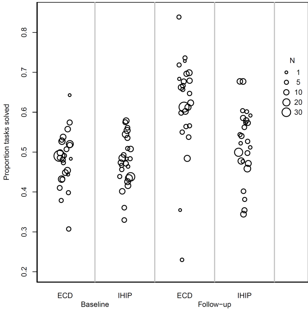
Figure S2: Proportion of tasks solved on cluster level. The mean proportion of tasks solved aggregated over all sub-domains and age groups are presented. Circle size indicates the number of children with a certain village.
