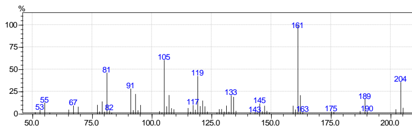
trans-Cadina-1(6),4-diene
