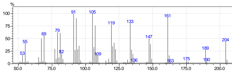
Cedrane
