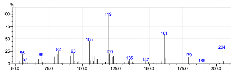
trans-Cadina-1(6),4-diene
