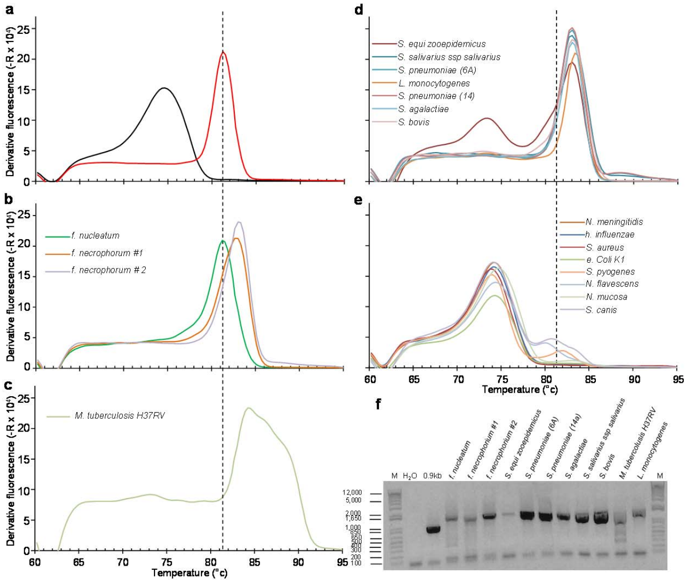
Figure S3: m16S qPCR detects a subset of bacteria in addition to Mollicutes with p_m16S(0.9kb) and water (a), detected (b-d) and non-detected (e) bacteria with amplicons sizes from panels a-d (f). Tm peak of 16S rDNA amplicon is indicated by the dotted line on each graph.
