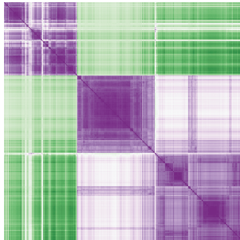
Transformed Correlations (C)
