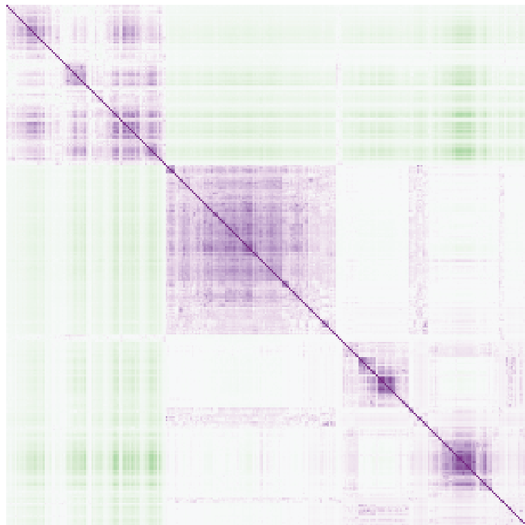
SparCC Correlations ( I_C )
