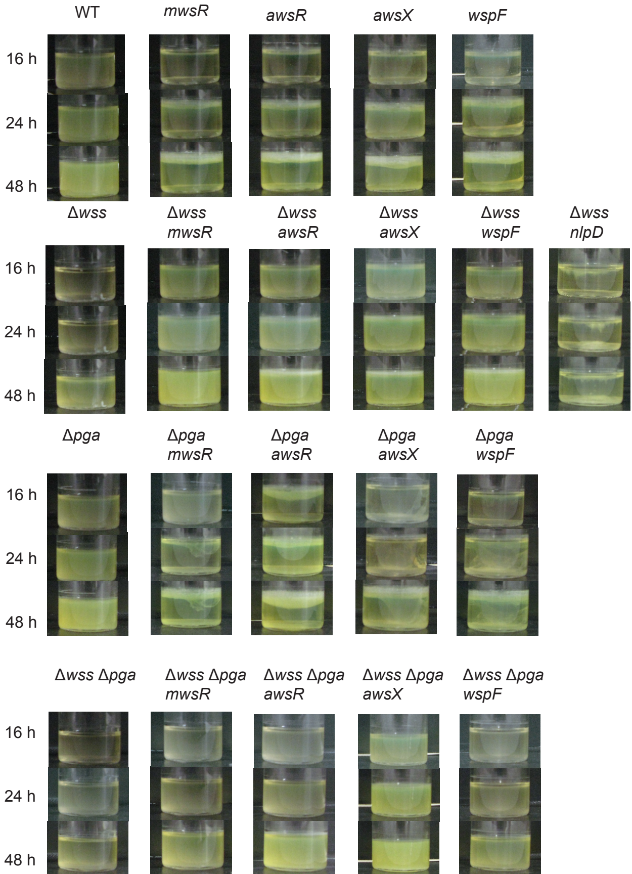
Figure S1. Growth in static microcosms of WS mutants in wild type background and without wss and/or pga .
