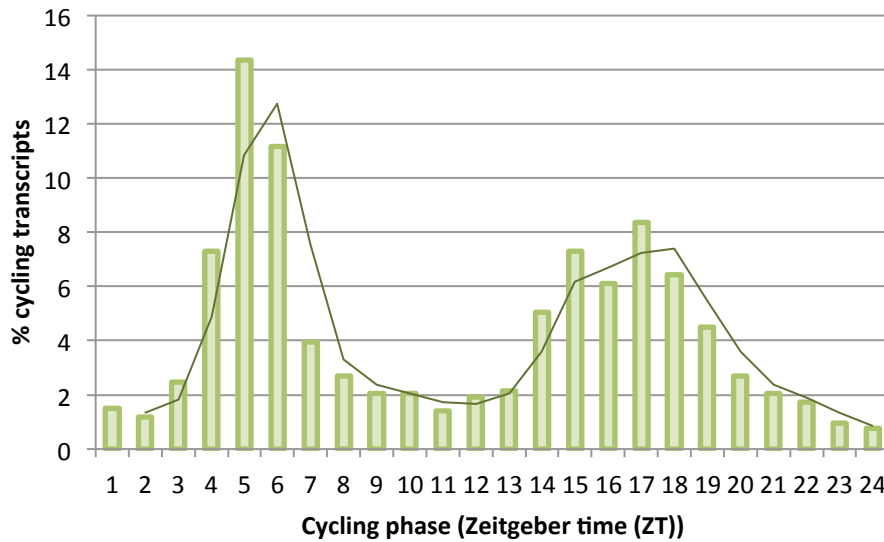
Supporting Figure 3. Bimodal phase distribution of transcripts cycling in LNvs is maintained when low-confidence (LC) as well as high-confidence (HC) cyclers are included. A total of ~900 HC and LC cycling transcripts are binned according to their peak expression (phase) and the percentage of all cycling transcripts in that bin is plotted. The shape of the distribution is emphasized by a trendline in the same color as the histogram. Phase shown was calculated by F24 analysis.
