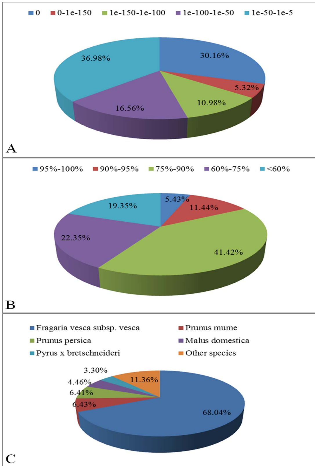
Figure S3. Characteristics of homology search of Taihangia unigenes against the NR database. The cutoff value was set at 1e-5 . (A) e value distribution of the top Blast hits for each unigene; (B) Similarity of the best Blast hits for each unigene; (C) Species distribution of the top Blast hits.
