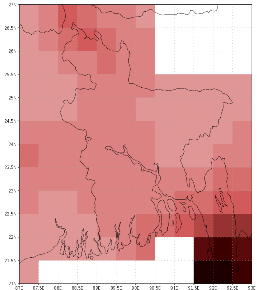
B Low Flood Years: June rainfall anomaly (mm/d)
