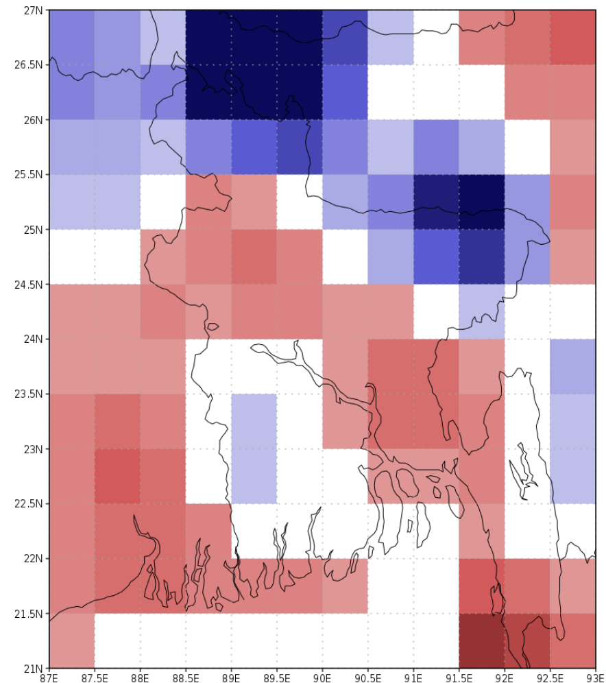
C June 2016 rainfall anomaly (mm/d)
