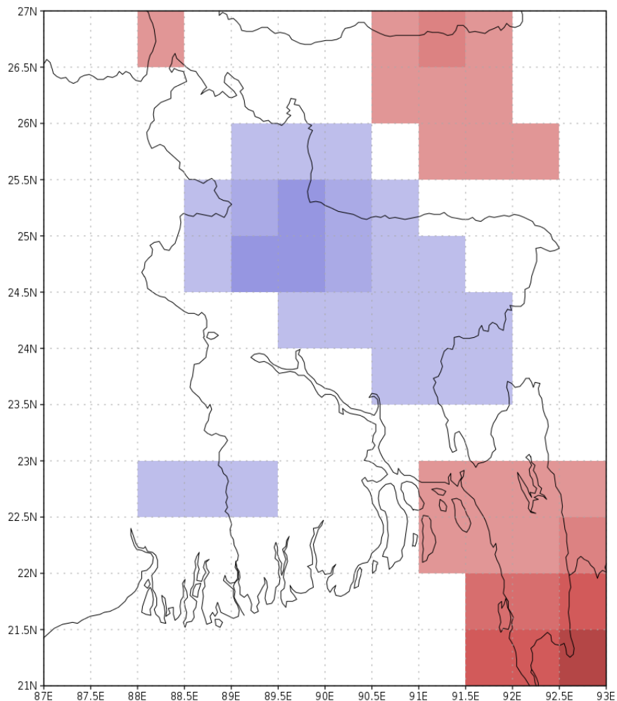
A High Flood Years: June rainfall anomaly (mm/d)
