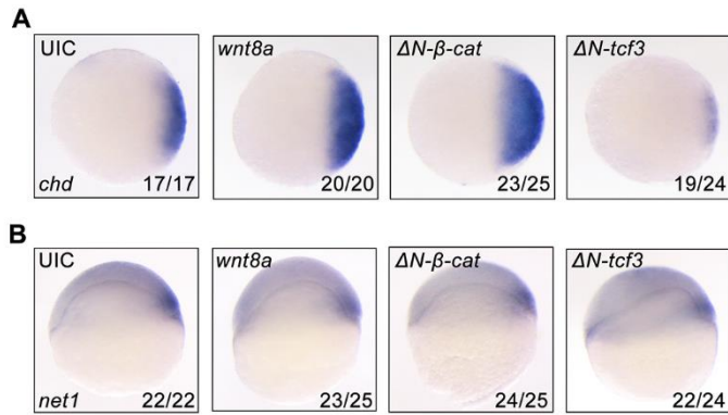
Figure S7 Zebrafish net1 expression is not regulated by Wnt/ \beta -catenin signaling. (A) The expression of chd , a well-known Wnt/ \beta -catenin signal responsive gene, in sphere stage embryos injected with 10 pg wnt8a mRNA, 50 pg \Delta N - \beta -catenin mRNA and 100 pg \Delta N - tcf3 mRNA, respectively. (B) The expression of net1 in 30%-epiboly stage embryos injected with indicated mRNAs. UIC, uninjected control. Note that the expression of net1 was not changed by either activation or inhibition of Wnt/ \beta -catenin signaling.
