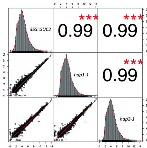
Figure S2 Pearson's coefficient plots for RNA-Seq of 35S::SUC2 , hdp1-1 and hdp2-1 .
