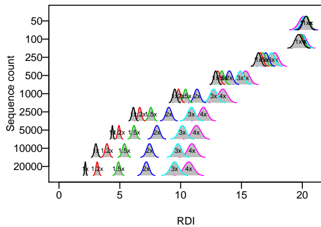
Genes = 1000
