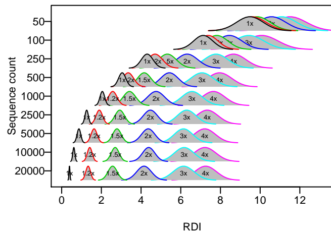
Genes = 500
