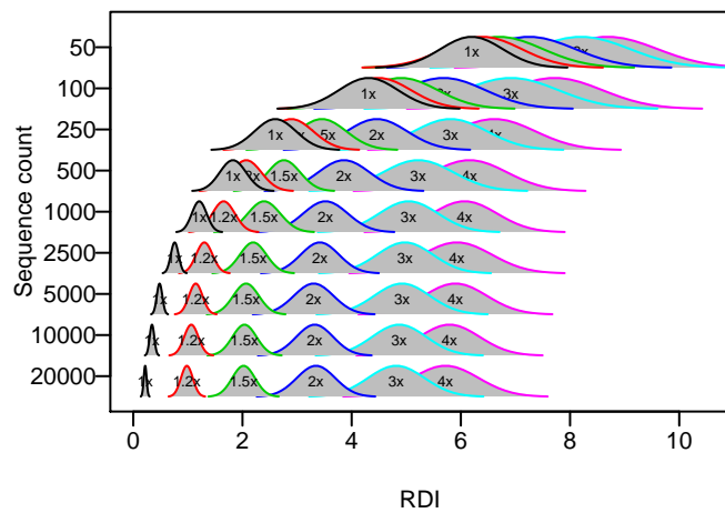
Genes = 100
