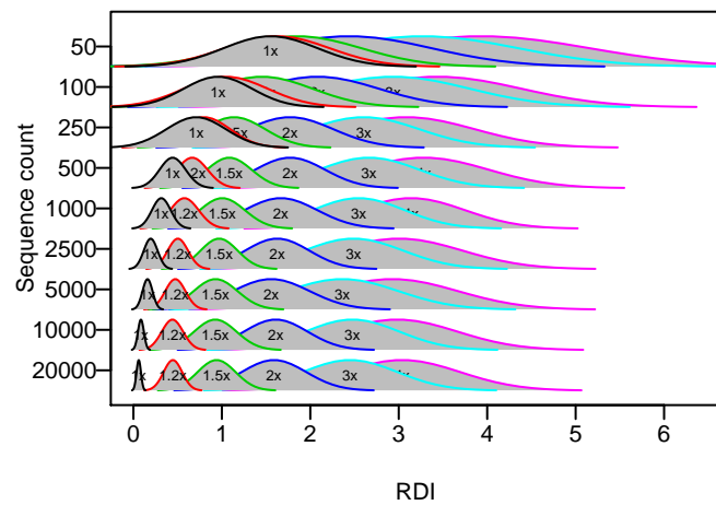
Genes = 50
