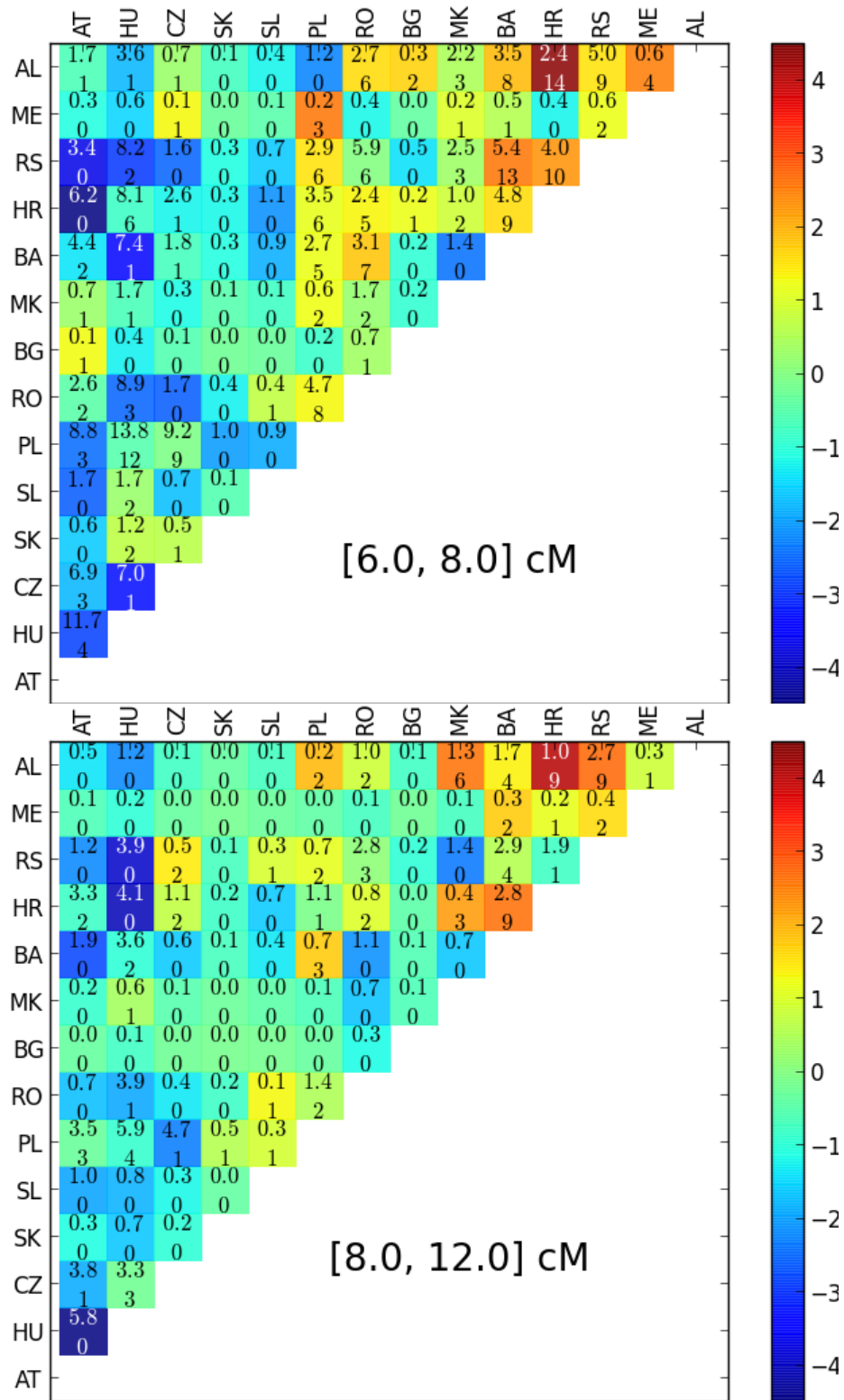
Figure S4: Residuals of best fit: As described in Fig. 10, residuals of the best fit for blocks of length 6 – 8 cM and 8 – 12 cM. AT: Austria, HU: Hungary, CZ: Czech Republic, SK: Slovakia, SL: Slovenia, PL: Poland, RO: Romania, BG: Bulgaria, MK: Macedonia, BA: Bosnia, HR: Croatia, RS: Serbia, ME: Montenegro, AL: Albania
