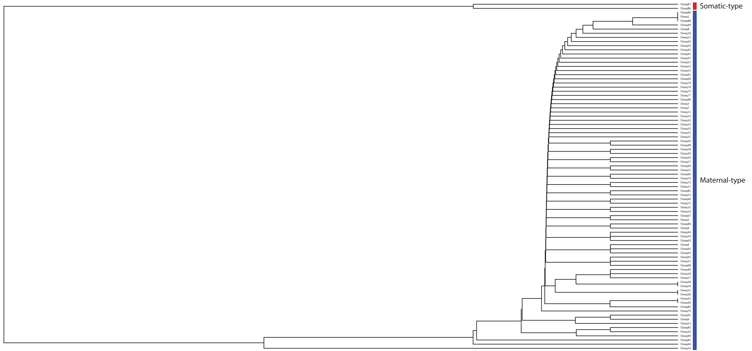
Supplemental Figure S4. Comparing the expressed 5S rRNA variant genes.
