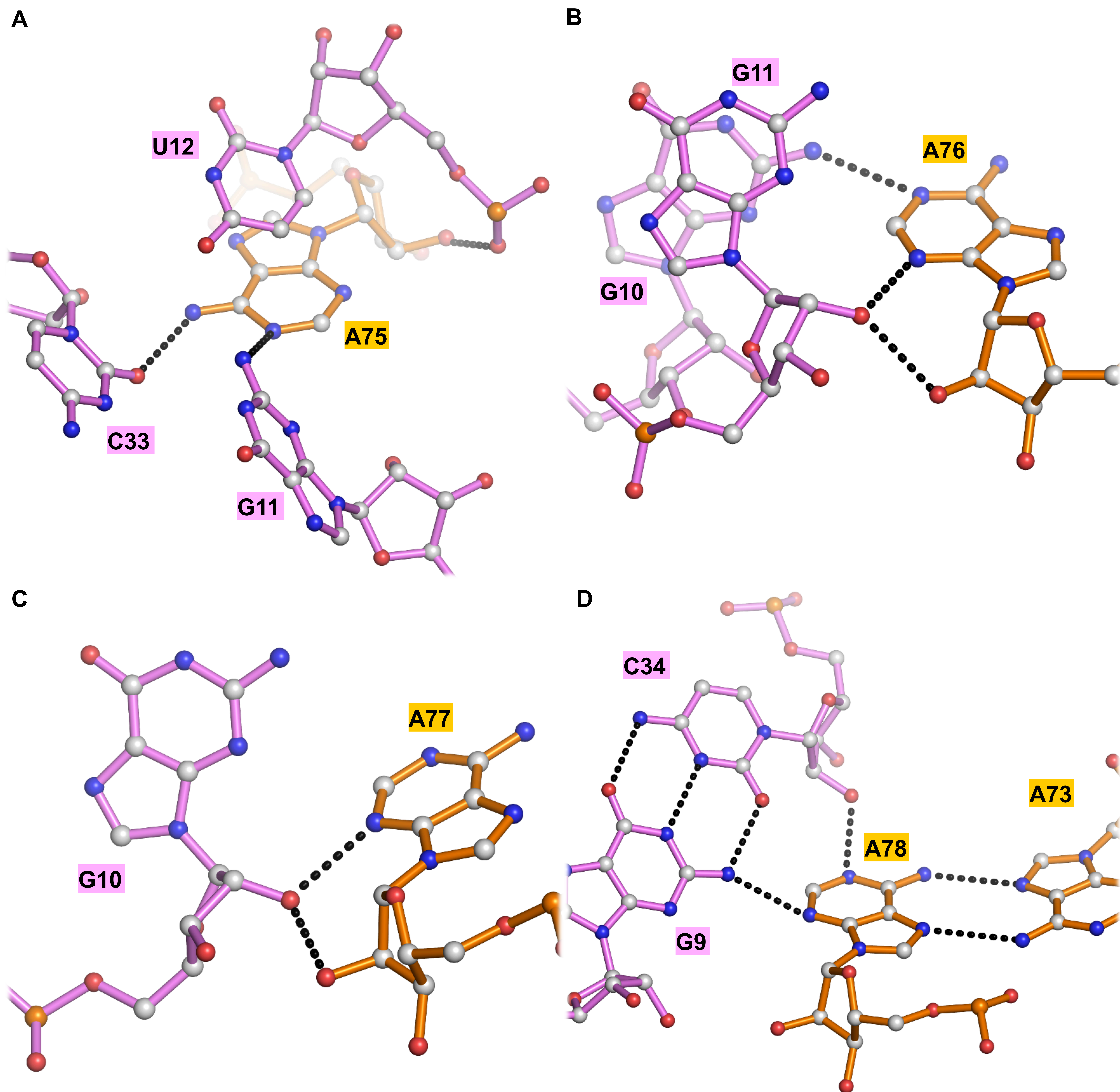
Figure S1. Individual Tertiary Interaction Between A-loop Residues and L1 Minor Groove (A) A75 (B) A76 (C) A77 (D) A78
