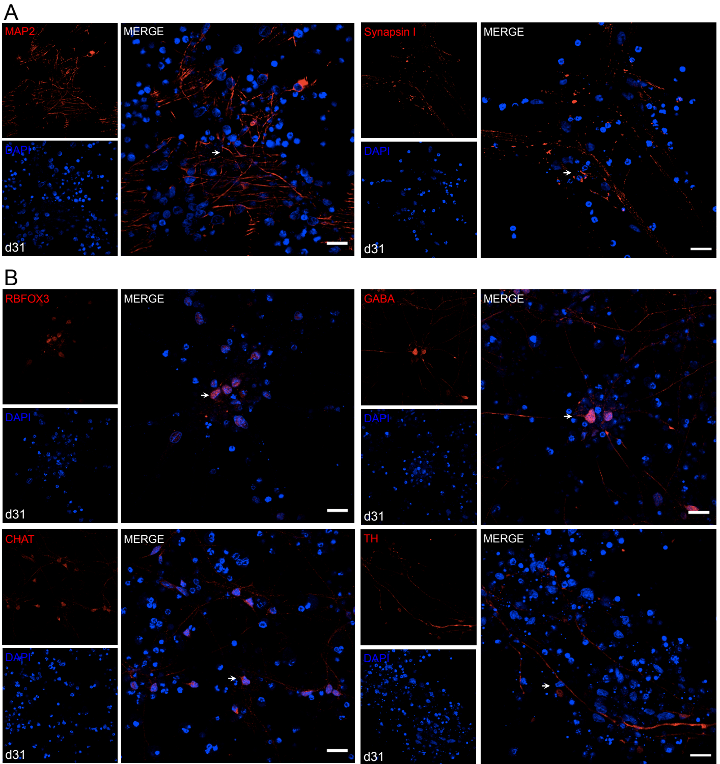
Supplemental Fig. 7. hESC-derived NPCs can differentiate to mature neuronal cells. (A) Representative quality controls on NPC-derived mature neuronal cells. A merged image of differentiated NPCs 31 days after initiation of differentiation and stained with an antibody against MAP2 (red, left panel) or Synapsin I (red, right panel); in both panels, nuclear DNA was stained with DAPI (blue). White bars, 20 mm. (B) Differentiated NPCs express neuron subtype specific markers. Shown are merged images of NPCs 31 days after initiation of differentiation and stained with an antibody against RBFOX3 (red, top left panel), GABA (red, top right panel), CHAT (red, bottom left panel) and TH (red, bottom right panel).
