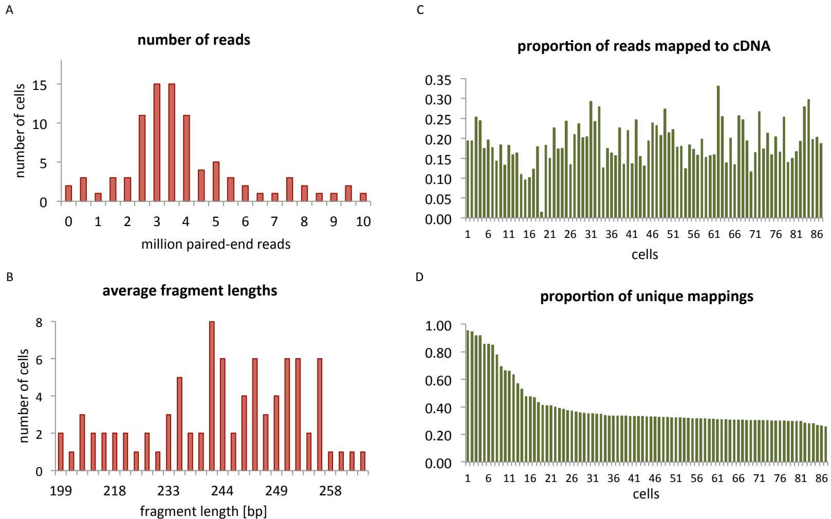
Figure S7: Detail of the single cell transcriptomes. A: the distribution of the read depths from different cells. Importantly, the ten smallest transcriptomes are all part of the largest clusters and thus do not affect the clustering. B: distribution of fragment length across cells. C: proportion of total reads mapping to known coding genes. D: average proportion of unique mappings.
