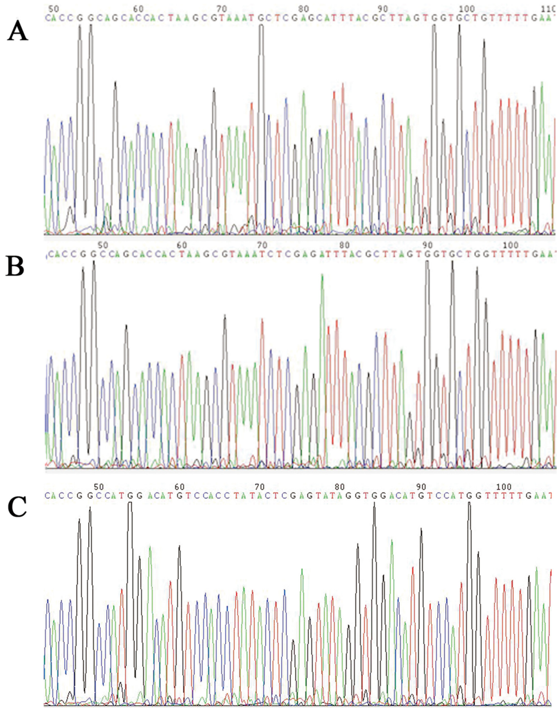
Supplementary Figure S1: DNA sequencing results of lentivirus PER1 -shRNA plasmids. A. PER1 -shRNA-I; B. PER1 -shRNA-II; C. PER1 -shRNA-III.
