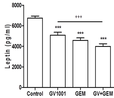
Supplementary Figure S2: Ghrelin and Leptin level among the different treatment groups. A. Ghrelin level was measured among the different treatment group B. Leptin level was measured among the different treatment group.
