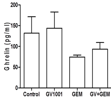
Supplementary Figure S2: Ghrelin and Leptin level among the different treatment groups. A. Ghrelin level was measured among the different treatment group B. Leptin level was measured among the different treatment group.
