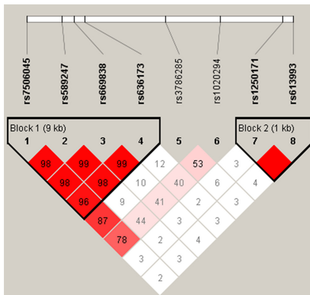
Supplementary Figure S1: Haplotype block map for SNPs in the IMPA2 gene.
