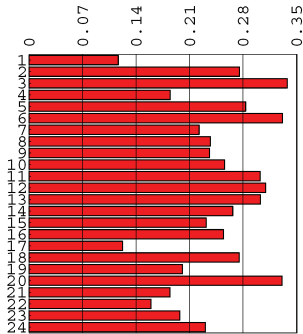
(a) SVD Basis Correlation
