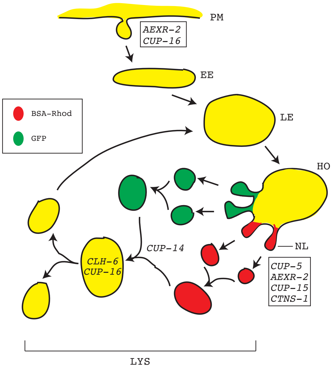
Figure S8 Model of novel CUP functions at the plasma membrane and endosomes. Shown is a simplified schematic of an endocytic pathway with presumed functions for the newly identified CUP proteins. EE = Early Endosome; HO = Hybrid Organelle; LE = Late Endosome; LYS = Lysosome; NL = Nascent Lysosome; PM = Plasma Membrane.
