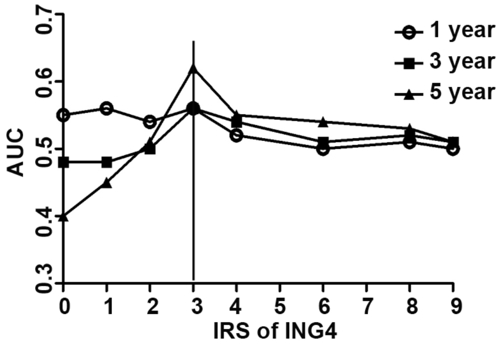
Supplementary Figure S3: ROC is obtained to determine the optimal cutoff value of ING4 expression. ROC obtains the area under the curves (AUCs) at different cutoff values of ING4 IRS for 1, 3 and 5 years of overall survival time
