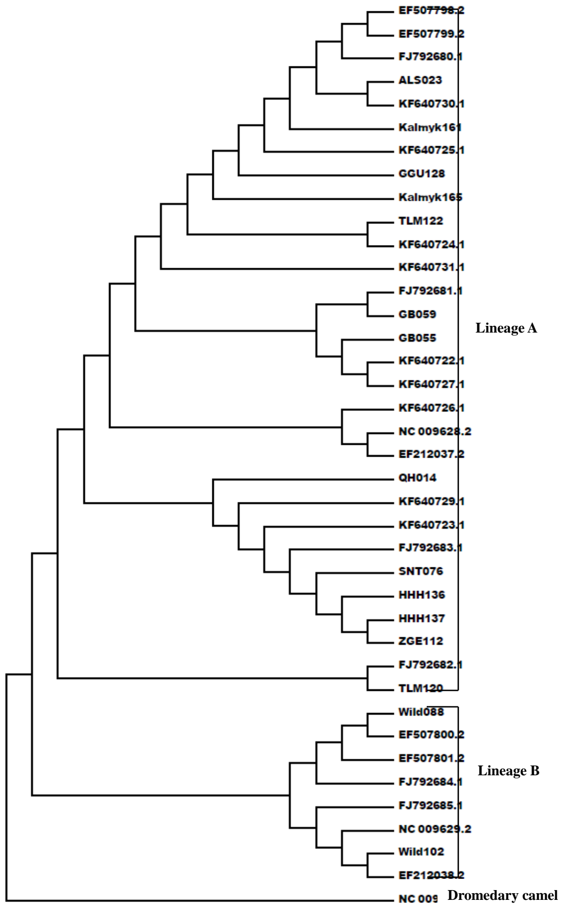
Figure S1 Neighbour-joining tree of wild and domestic Bactrian camel haplotypes based on 809 bp of the mtDNA. Haplotypes are grouped in two main lineages (lineage A and lineage B), each showing subgroupings.
