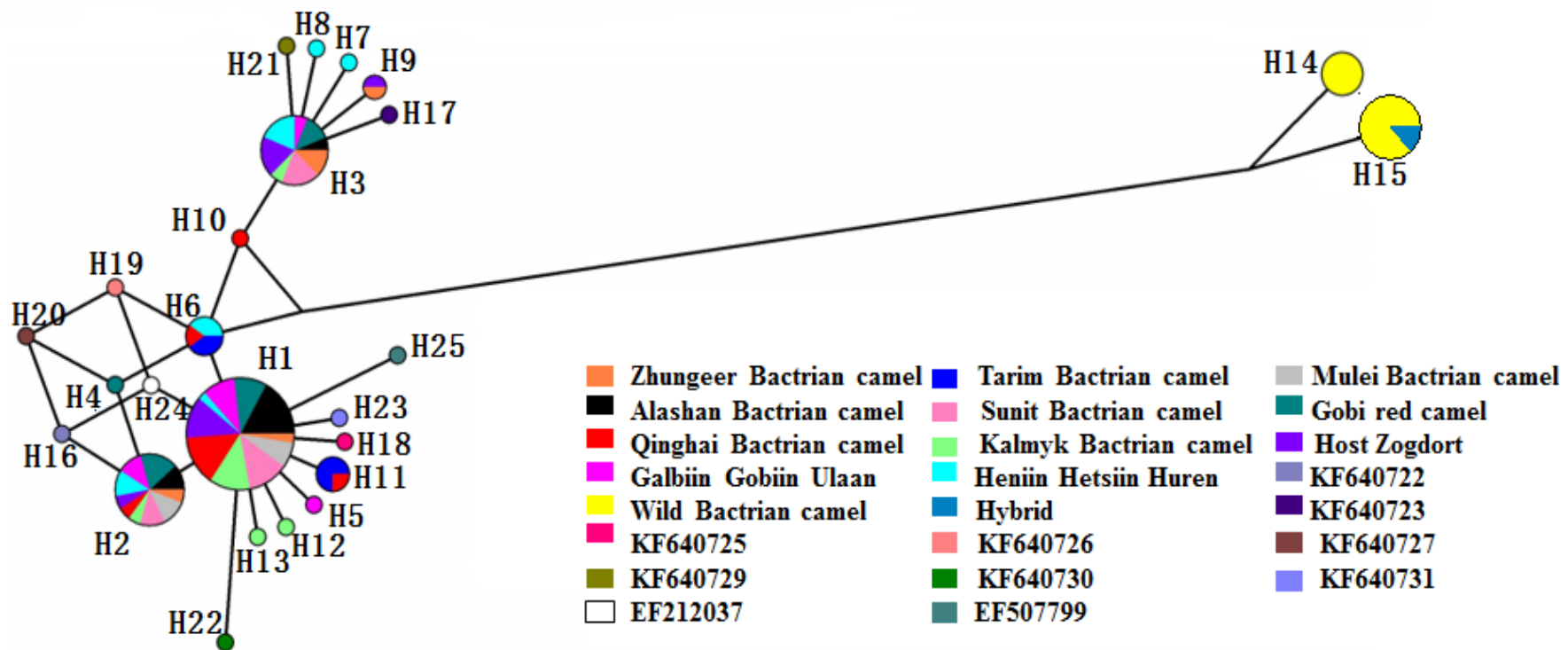
Figure S2 Median-joining network of 25 mtDNA haplotypes of domestic and wild Bactrian camels. The area of the circle is proportional to haplotype frequency.
