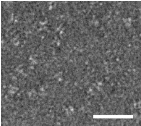
Arp2/3 + Crn1-GST
