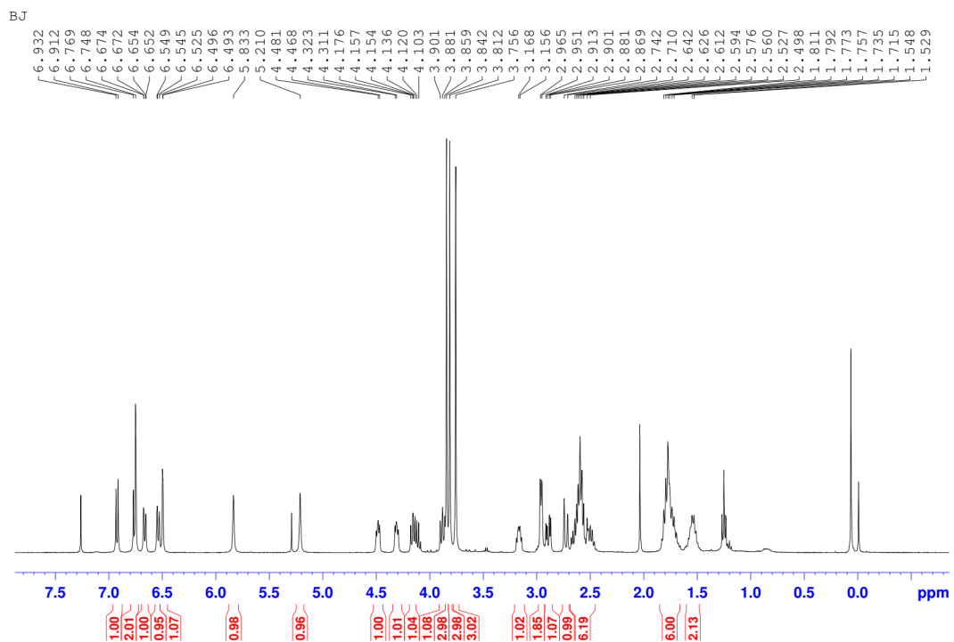
Supplementary Figure S1: Nuclear magnetic resonance analysis of Biotin-Atn.
