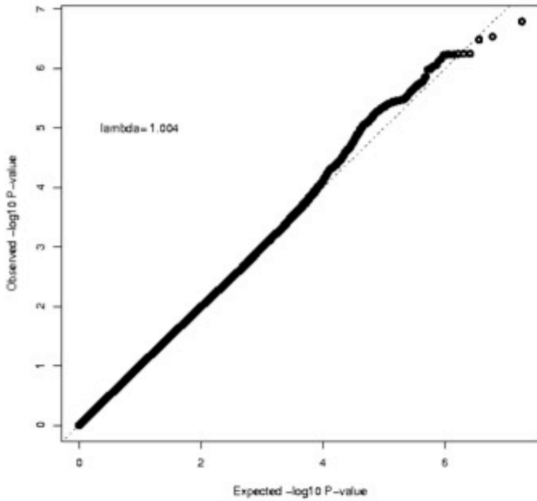
S6a Fig. QQ-plot for GWAS analysis of venous on the Illumina Omniexpress platform (406 cases and 4,786 controls).
