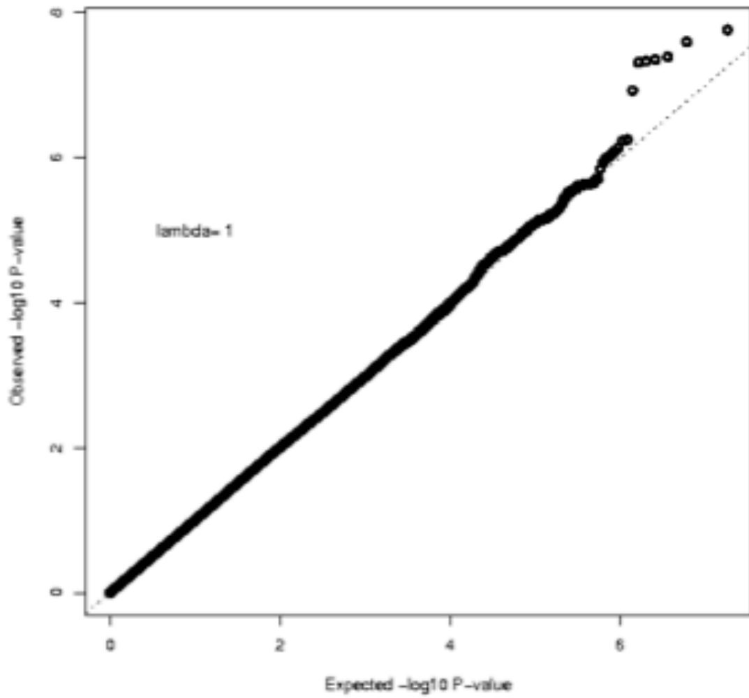
S6c Fig. QQ-plot for GWAS analysis of venous on the Affymetrix platform (532 cases and 7,147 controls).
