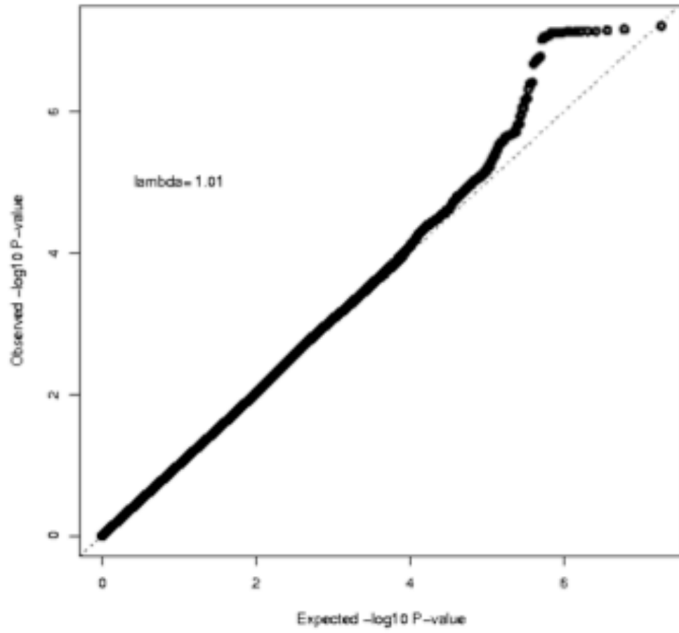
S6b Fig. QQ-plot for GWAS analysis of venous on the Illumina Omniexpress platform (406 cases and 4,786 controls).
