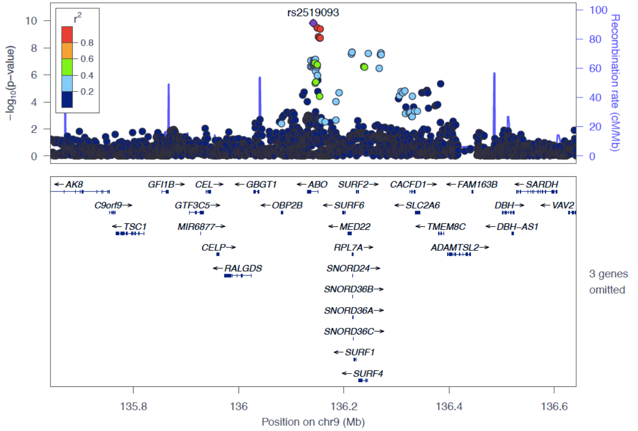
S7b Fig. LocusZoom plot for the VTE ABO locus.
