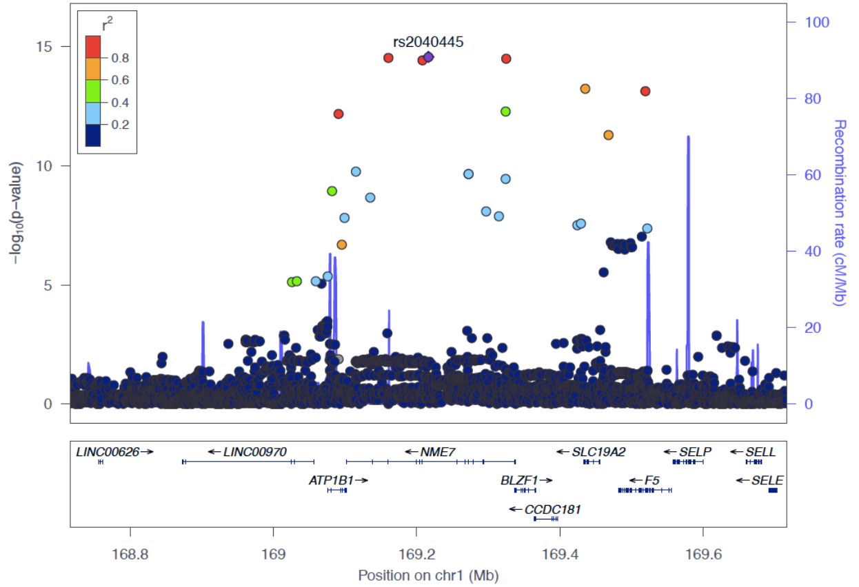
S7a Fig. LocusZoom plot for the VTE F5 locus.
