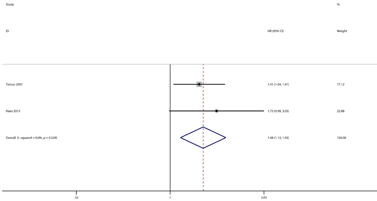
Supplementary Figure 2: Meta-analysis with a random-effect model for the association between GLUT-1 and OS in gastric cancer.
