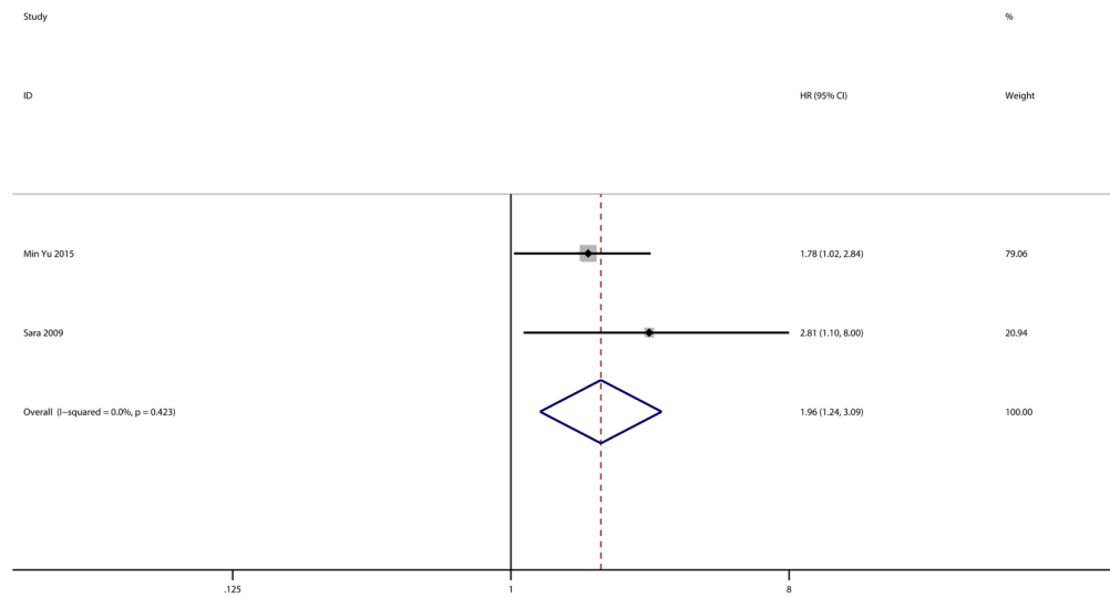
Supplementary Figure 1: Meta-analysis with a random-effect model for the association between GLUT-1 and OS in pancreatic cancer.
