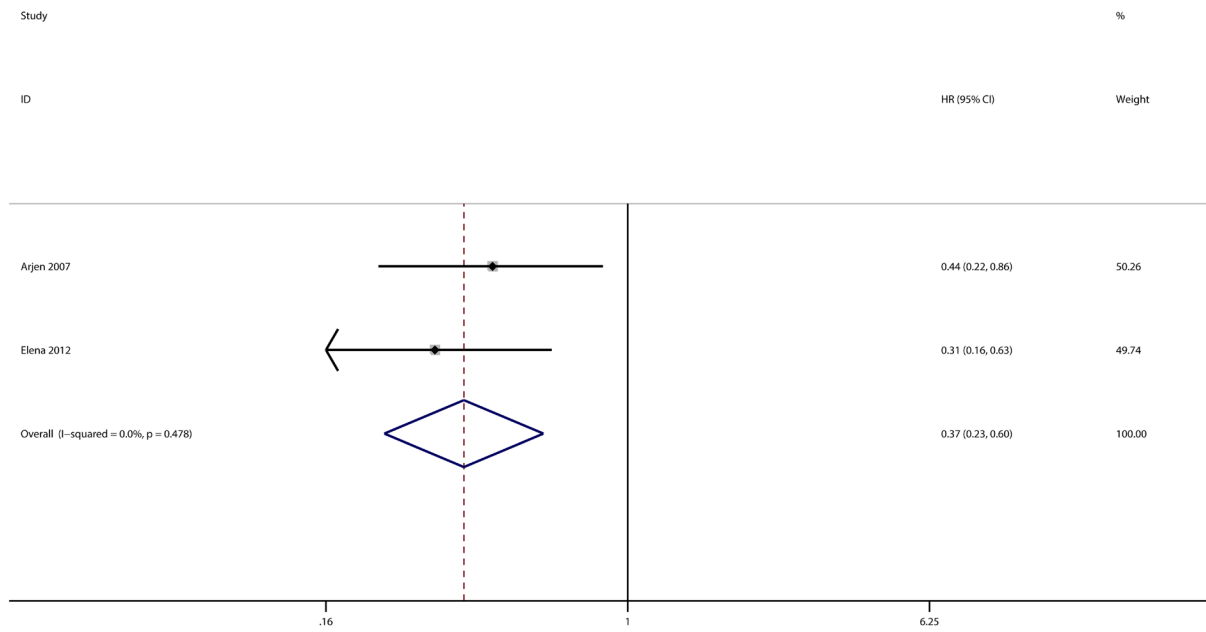
Supplementary Figure 3: Meta-analysis with a random-effect model for the association between GLUT-1 and OS in colorectal cancer.
