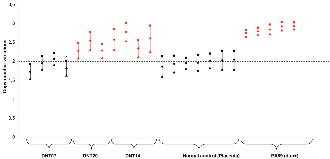
Supplementary Figure S1: DDPCR™ inter-assays reproducibility.
