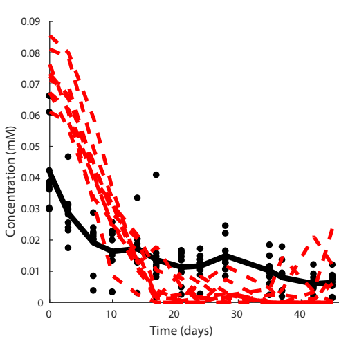
Predicted udpg[c]
