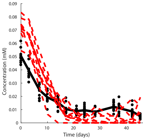
Predicted ins[c]
