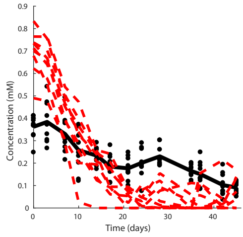
Predicted r5p[c]
