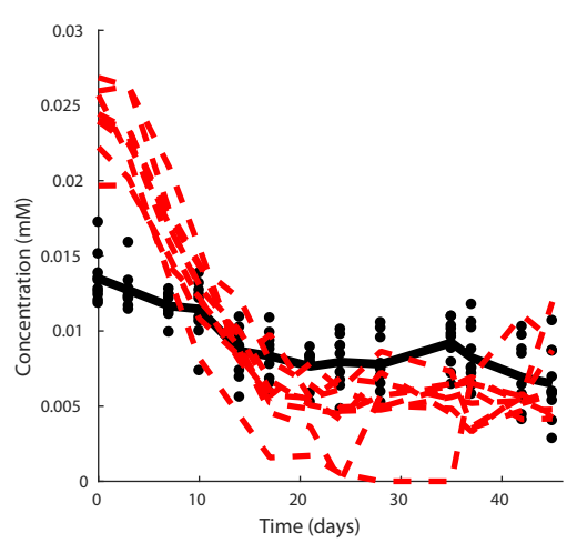
Predicted xu5p-D[c]
