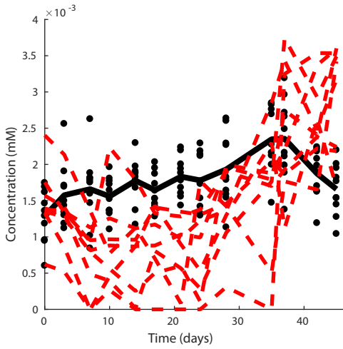
Predicted ru5p-D[c]
