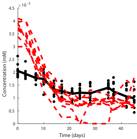
Predicted udpg[c]
