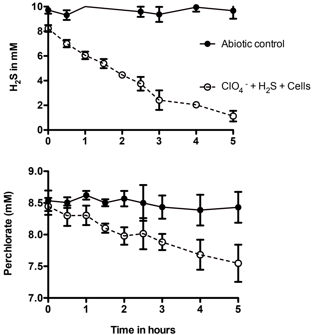
Figure S1. H 2 S oxidation with concomitant perchlorate reduction. PS cultures showing H 2 S oxidation (top panel) is coupled to perchlorate reduction (bottom panel) in absence of other electron donors.
