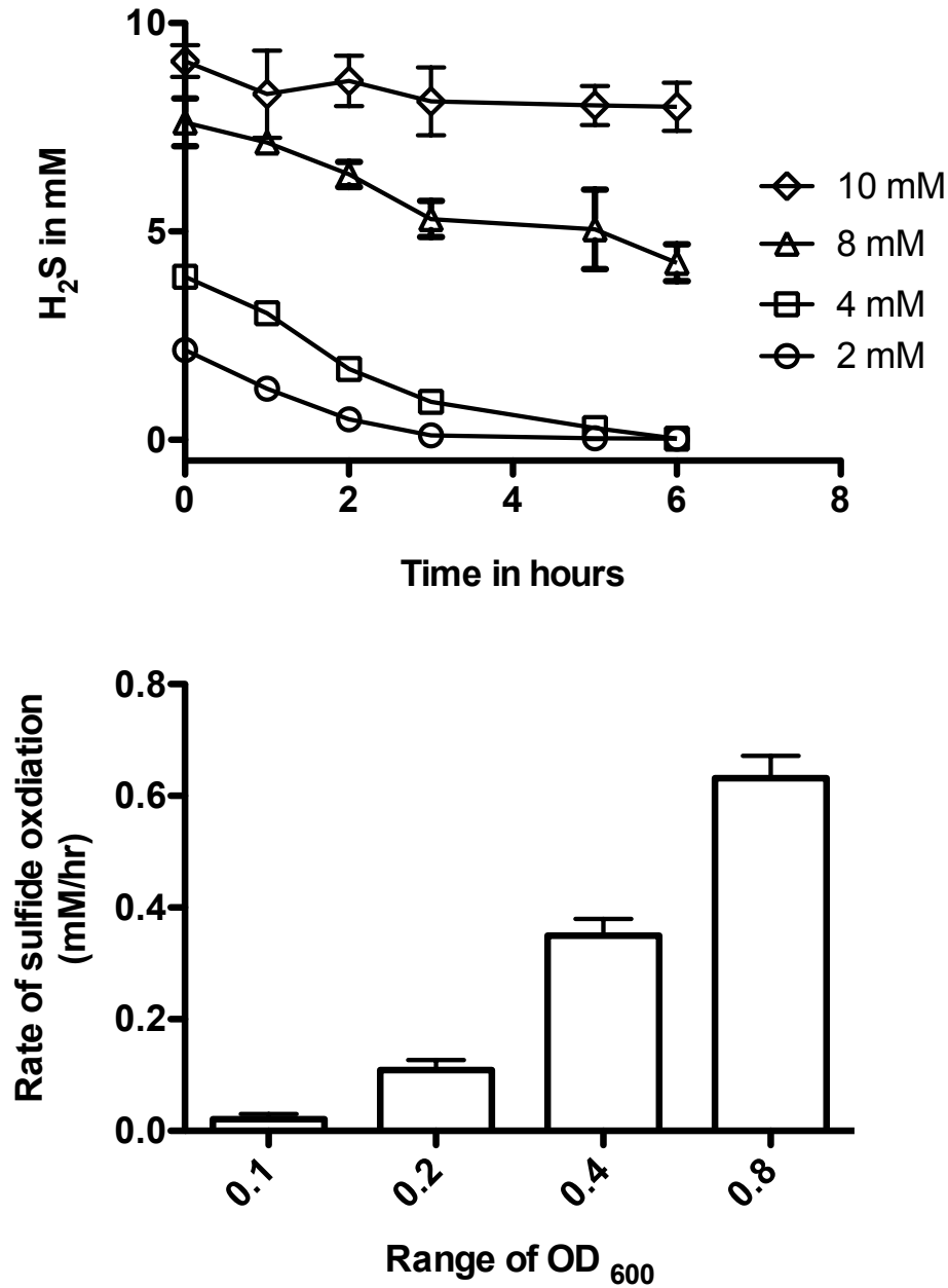
Figure S2 H 2 S oxidation is directly proportional to cell density. The rate of H 2 S oxidation is dependent on the concentration of H 2 S and cell OD, faster rates are observed for lower concentrations of H 2 S with high cell OD.
