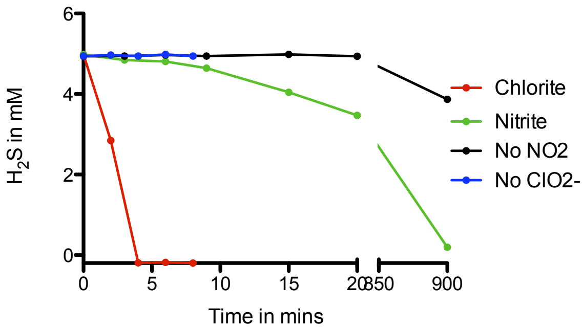
SI Figure 3. Abiotic H 2 S oxidation with chlorite and nitrite in comparison to controls.
