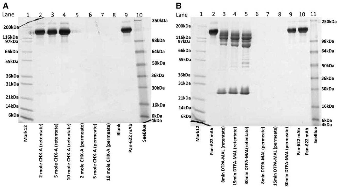
SUPPLEMENTARY FIG. S1. Structural evaluation of PAN-622 conjugates: (A) nonreducing SDS-PAGE of PAN-622 CHX-A' conjugates; (B) nonreducing SDS-PAGE of PAN-622 DTPA-MAL conjugates. SDS-PAGE, sodium dodecyl sulfate/polyacrylamide gel electrophoresis.
