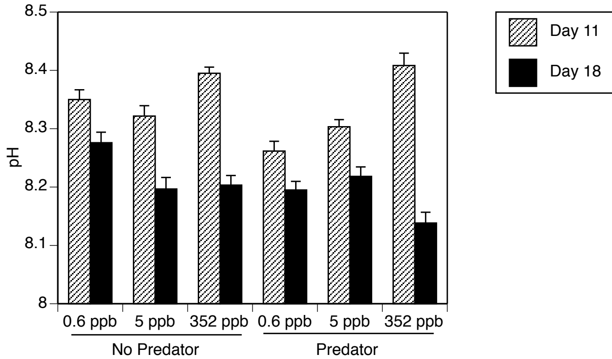
3 S2 Figure. pH measurements for the two sampling periods (days 11 and 18 of the 4 experiment). Time periods are represented by patterns denoted in the figure legend. Data are 5 means + 1 SE.
