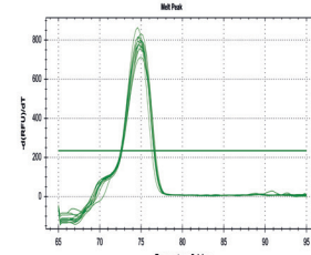
EpMADS12 FUL
