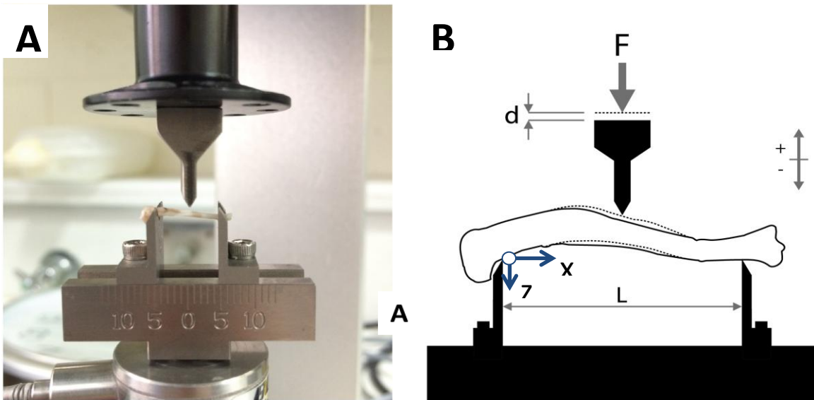
Supplementary Figure 1. (A) A photograph of the actual set up of the Bose Biodynamic 5500 Test Instrument. (B) A schematic representation of the 3-point bending apparatus where, F = applied load (in z -direction), L = distance (in x -direction) between supports, d = displacement/deformation of the bone (in z -direction).
