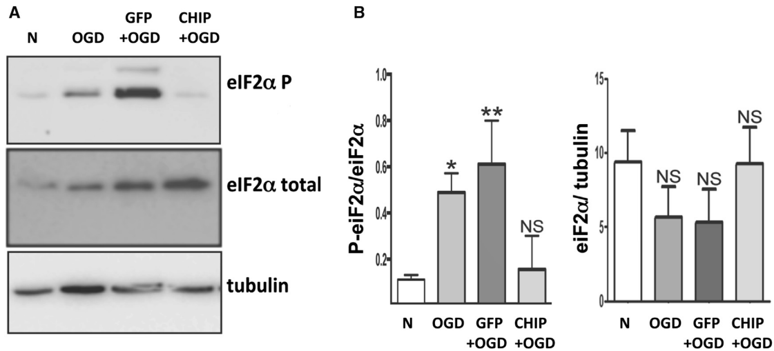
Figure 3. CHIP Overexpression Prevents eIF2 \alpha Phosphorylation Induced by Oxygen and Glucose Deprivation after 24 hr of Reperfusion In Vitro
