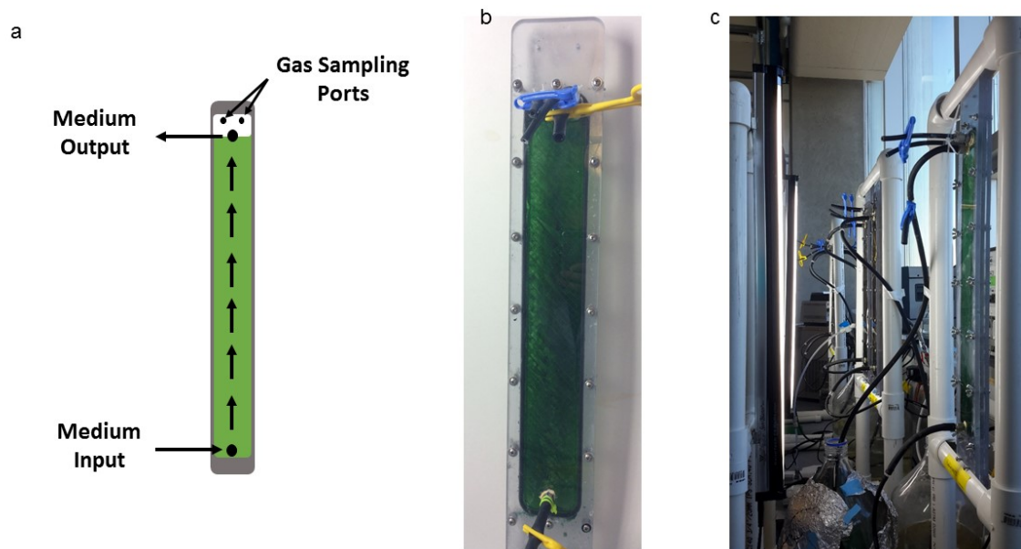
Figure S3. Design of the flat panel photobioreactor system showing (a) a schematic of the photobioreactor design and media flow pattern, (b) a photo of an individual photobioreactor, and (c) a photo of the photobioreactor system in operation.
