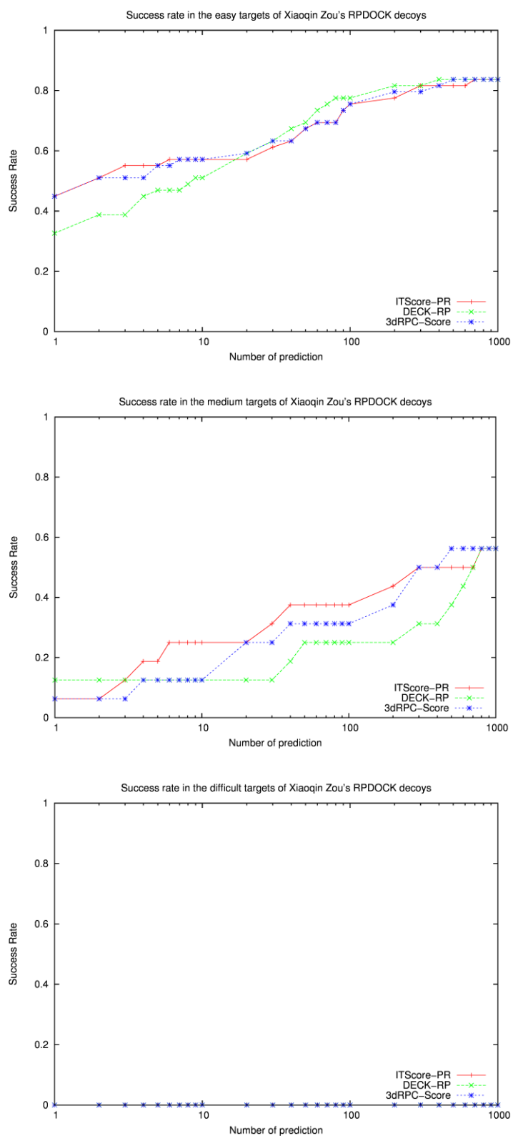
S1 Fig. The success rates for easy, medium and difficult targets in Zou's benchmark by RPDOCK.
