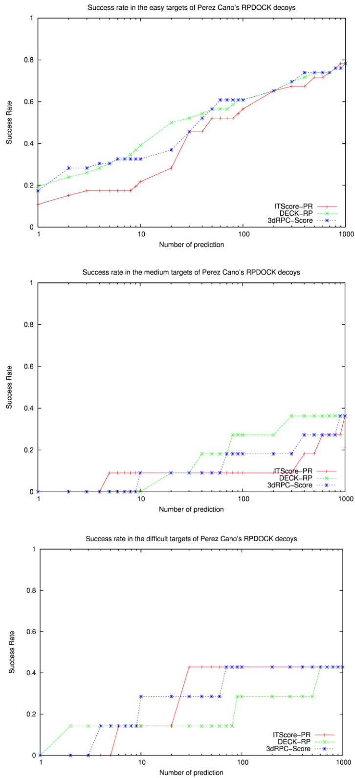
S3 Fig. The success rates for easy, medium and difficult targets in Perez Cano's benchmark by RPDOCK.
