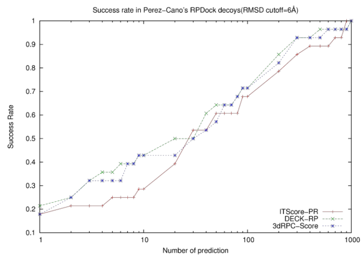
S4 Fig. The success rate in three testing sets, when the near-native cutoff is RMSD=6Å.
